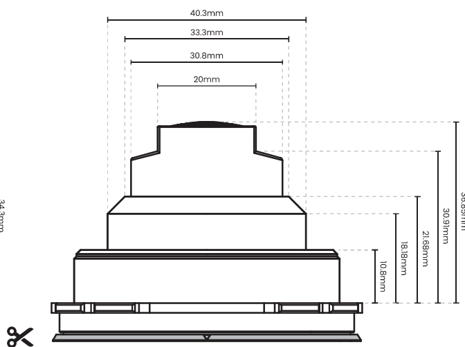
12mm T2.9 Lite Zero-D VV Cine
